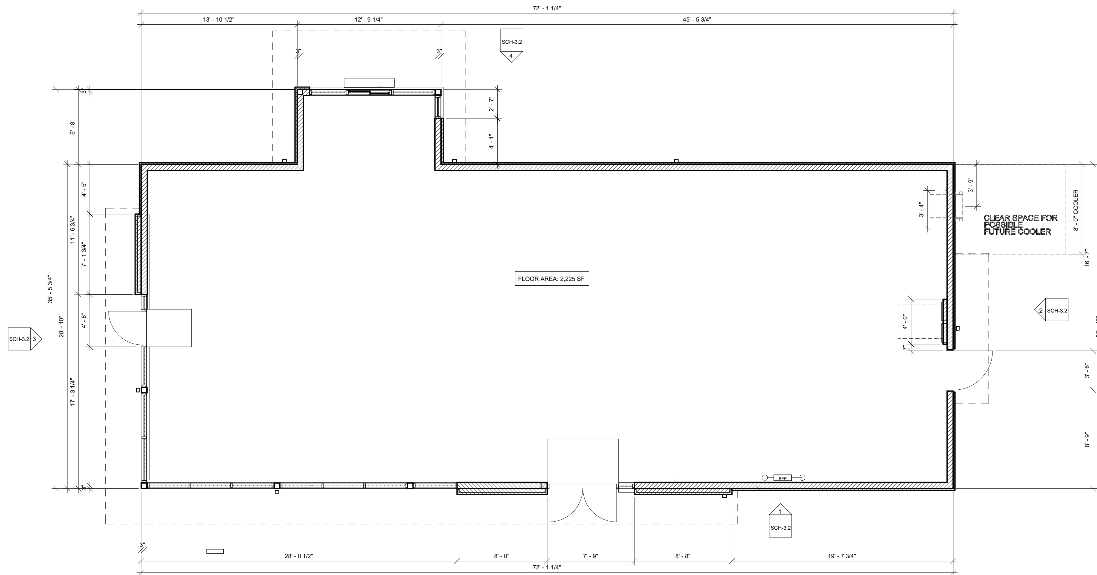
PROPOSED STARBUCKS CAFE SHELL FLOOR PLAN SCALE: 3/16" = 1'-0"
