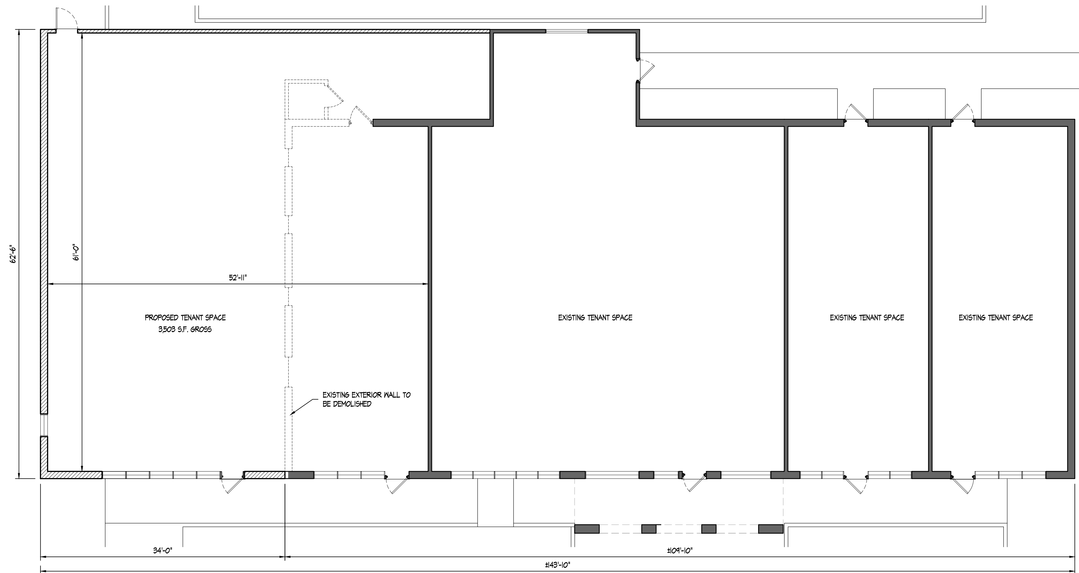
1 PROPOSED MEDICAL BLDG. FIRST FLOOR PLAN SCALE: 1/8" = 1'-0"
